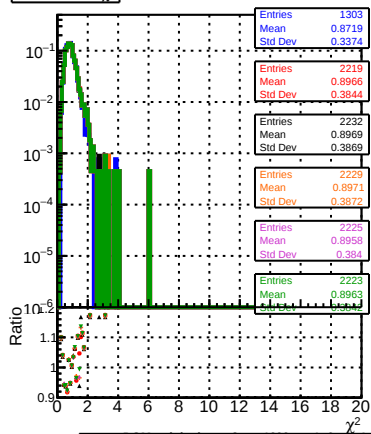
normalized \chi^2
