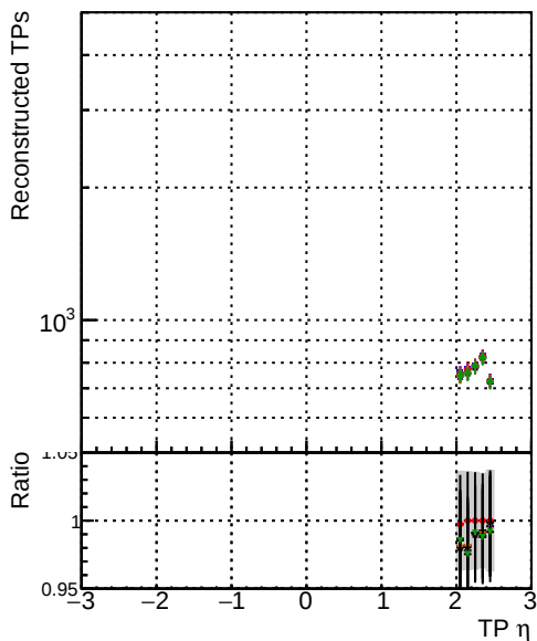
to2p5 pt0b1to1 eta2p0to2p5 pt0b1to1-eta2p0to2p5 pt0b1to1-eta2p0to2p5 pt0b1to1-eta2p0to2p5 pt0b1to1 eta2p0to2p5
