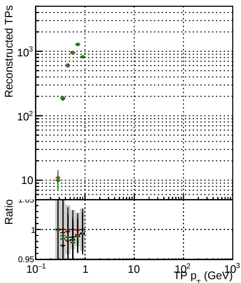
to2p5 pt0b1to1 eta2p0to2p5 pt0b1to1-eta2p0to2p5 pt0b1to1-eta2p0to2p5 pt0b1to1-eta2p0to2p5 pt0b1to1 eta2p0to2p5
