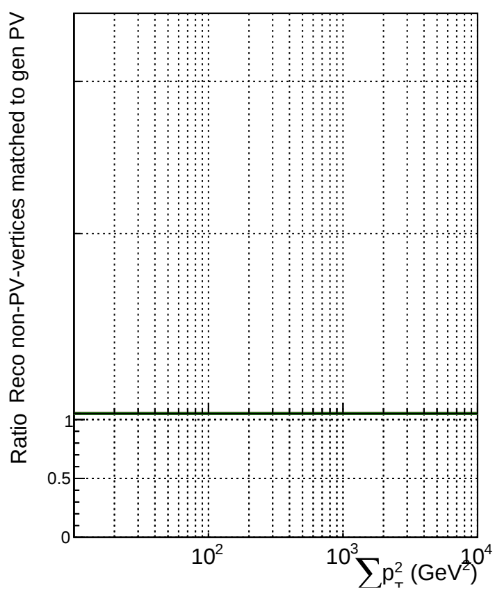
RecoAssoc2GenPVMatchedNotHighest_Pt2
