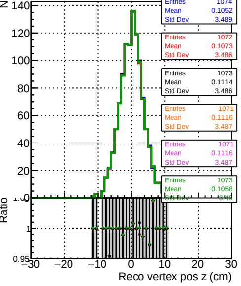
ReconstructedAllAssoc2Gen_Z
