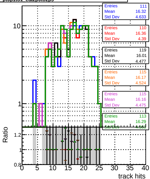
Legend: BDM original, BDM pixel, BDM template, BDM cutChiSquare, BDM eta2p0to2p5, BDM pixel, BDM template, BDM cutChiSquare, BDM eta2p0to2p5, BDM pixel, BDM template, BDM cutChiSquare, BDM eta2p0to2p5, BDM pixel, BDM template, BDM cutChiSquare, BDM eta2p0to2p5
