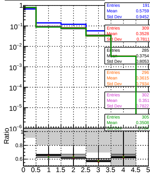
mean hits
