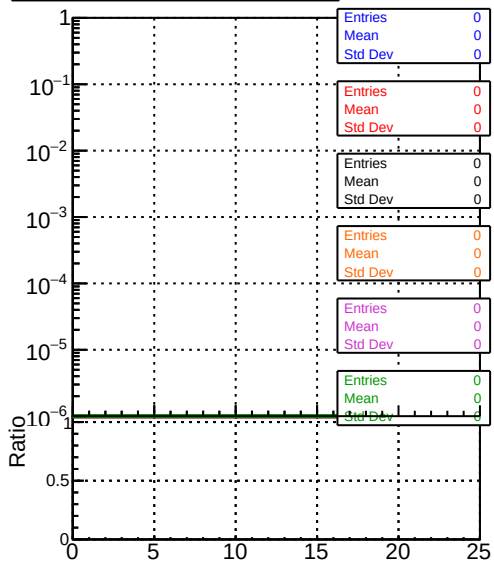
Legend for mean hits vs \eta : blue: BQM original step2 eta2p0to2p5 red: BQM original step2 eta2p0to2p5 orange: BQM original step2 eta2p0to2p5 purple: BQM original step2 eta2p0to2p5 green: BQM original step2 eta2p0to2p5 blue: BQM pixel CDDT template CutChiSquare10 step2 eta2p0to2p5 red: BQM pixel CDDT template CutChiSquare10 step2 eta2p0to2p5 orange: BQM pixel CDDT template CutChiSquare10 step2 eta2p0to2p5 purple: BQM pixel CDDT template CutChiSquare10 step2 eta2p0to2p5 green: BQM pixel CDDT template CutChiSquare10 step2 eta2p0to2p5
