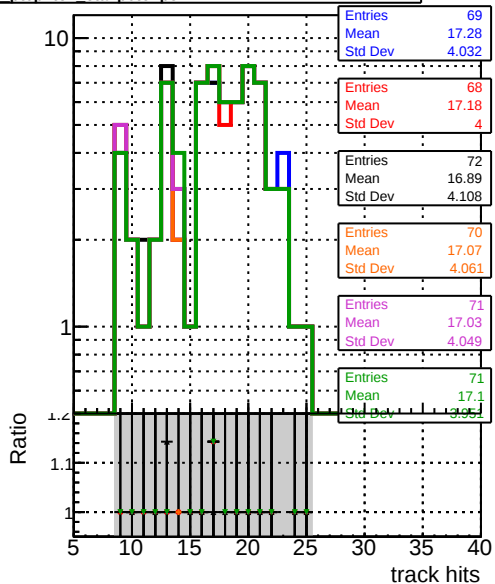
mean hit Legend: BQM original, BQM pixel, BQM CDD, BQM CDD+Template, BQM CDD+Template+ChiSquare, BQM CDD+Template+ChiSquare+step2, BQM CDD+Template+ChiSquare+step2+eta2p0to2p5, BQM CDD+Template+ChiSquare+step2+eta2p0to2p5+eta2p0to2p5
