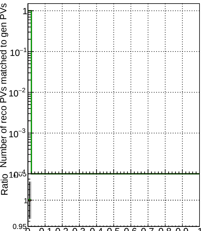
RecoPVAssoc2GenPVMatched_Purity
