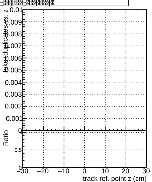
pt0p1to1_eta2p0to2p5 pt0p1to1_eta2p0to2p5
