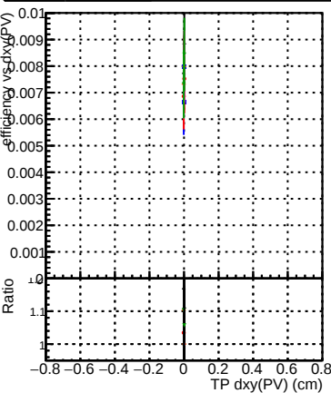
Efficiency vs Dxy(PV) DOM original step2 pt0pt01 eta1p6to2p0 DOM pixelCPETemplate step2 pt0pt01 eta1p6to2p0 DOM pixelCPETemplateCutChiSquare10 step2 pt0pt01 eta1p6to2p0 DOM pixelCPETemplateCutChiSquare15 step2 pt0pt01 eta1p6to2p0 DOM pixelCPETemplateCutChiSquare20 step2 pt0pt01 eta1p6to2p0 DOM pixelCPETemplateCutChiSquare30 step2 pt0pt01 eta1p6to2p0
