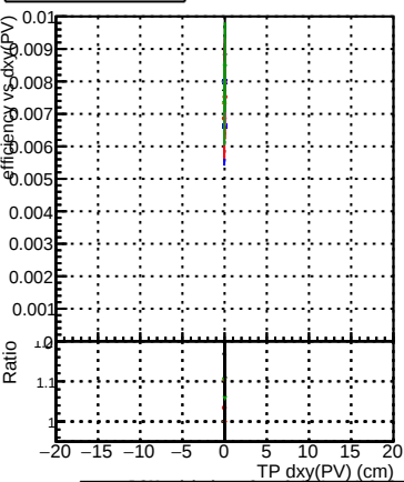
Efficiency vs Dxy(PV) DOM original step2 pt0pt01 eta1p6to2p0 DOM pixelCPETemplate step2 pt0pt01 eta1p6to2p0 DOM pixelCPETemplateCutChiSquare10 step2 pt0pt01 eta1p6to2p0 DOM pixelCPETemplateCutChiSquare15 step2 pt0pt01 eta1p6to2p0 DOM pixelCPETemplateCutChiSquare20 step2 pt0pt01 eta1p6to2p0 DOM pixelCPETemplateCutChiSquare30 step2 pt0pt01 eta1p6to2p0
