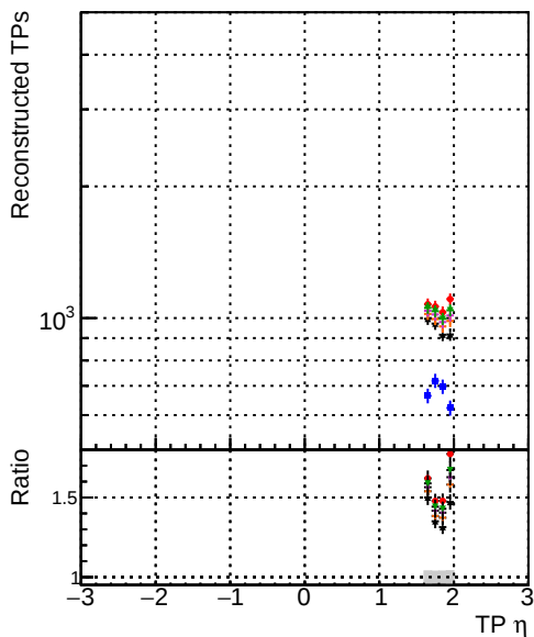
DEM original step2 p10p10t1 et1p6t2p0 DEM pixe10p10t1 et1p6t2p0 DEM pixe20p10t1 et1p6t2p0 DEM pixe50p10t1 et1p6t2p0 DEM pixe100p10t1 et1p6t2p0 DEM pixe200p10t1 et1p6t2p0 DEM pixe500p10t1 et1p6t2p0 DEM pixe1000p10t1 et1p6t2p0
