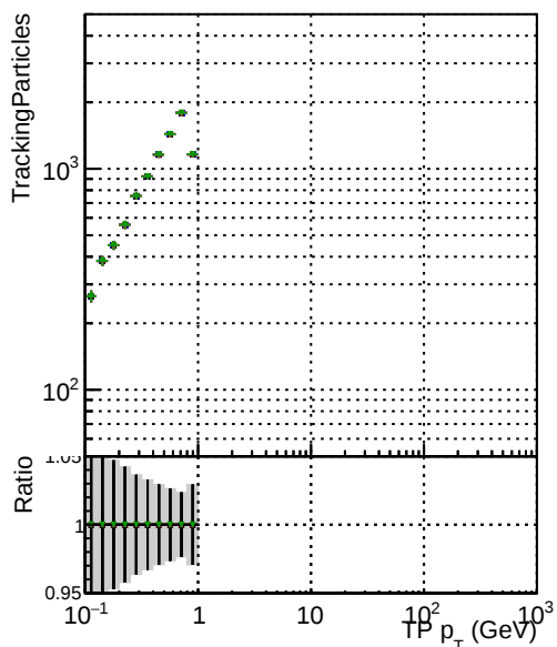
DEM original step2 p10p10t1 et1p6t2p0 DEM pixe10p10t1 et1p6t2p0 DEM pixe20p10t1 et1p6t2p0 DEM pixe50p10t1 et1p6t2p0 DEM pixe100p10t1 et1p6t2p0 DEM pixe200p10t1 et1p6t2p0 DEM pixe500p10t1 et1p6t2p0 DEM pixe1000p10t1 et1p6t2p0
