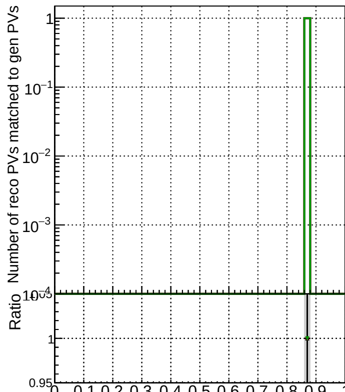
RecoPVAssoc2GenPVMatched_Purity
