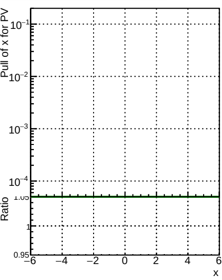
RecoPVAssoc2GenPVMatched_PullX
