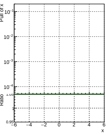
RecoAllAssoc2GenMatched_PullX
