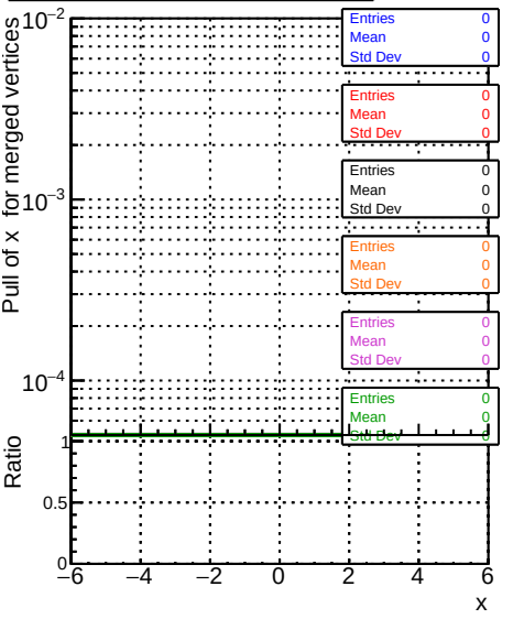
RecoAllAssoc2GenMatchedMerged_PullX
