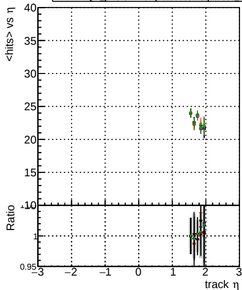
Legend for mean hits vs track \eta : DDV original DDV original step2 DDV original step2 eta1p6to2p0 DDV pixel DDV pixel template DDV pixel template cutChiSquare10 DDV pixel template cutChiSquare10 step2 DDV pixel template cutChiSquare10 eta1p6to2p0 DDV pixel template cutChiSquare20 DDV pixel template cutChiSquare20 step2 DDV pixel template cutChiSquare20 eta1p6to2p0 DDV pixel template cutChiSquare30 DDV pixel template cutChiSquare30 step2 DDV pixel template cutChiSquare30 eta1p6to2p0
