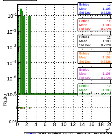
normalized \chi^2
