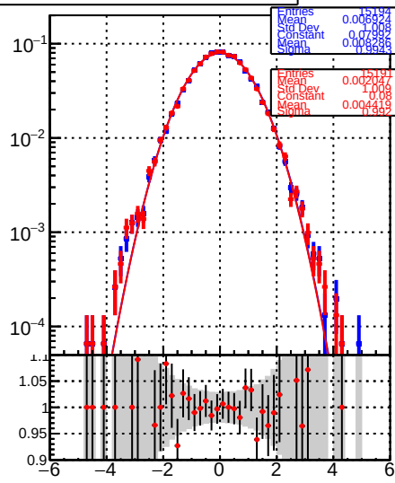
RecoAllAssoc2GenMatchedMerged_PulIZ
