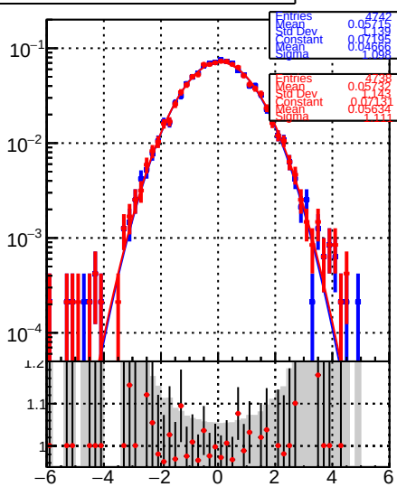
RecoPVAssoc2GenPVMatched_PulIX
