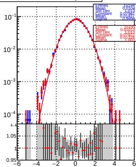
RecoAllAssoc2GenMatchedMerged_PulIX
