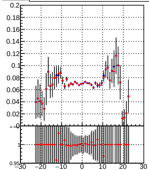
Efficiency vs. sim PV z Legend: DQM_TT_mkFit-DQM_ (Blue line with error bars) DQM_TT_mkFitRETEST-DQM_ (Red line with error bars)
