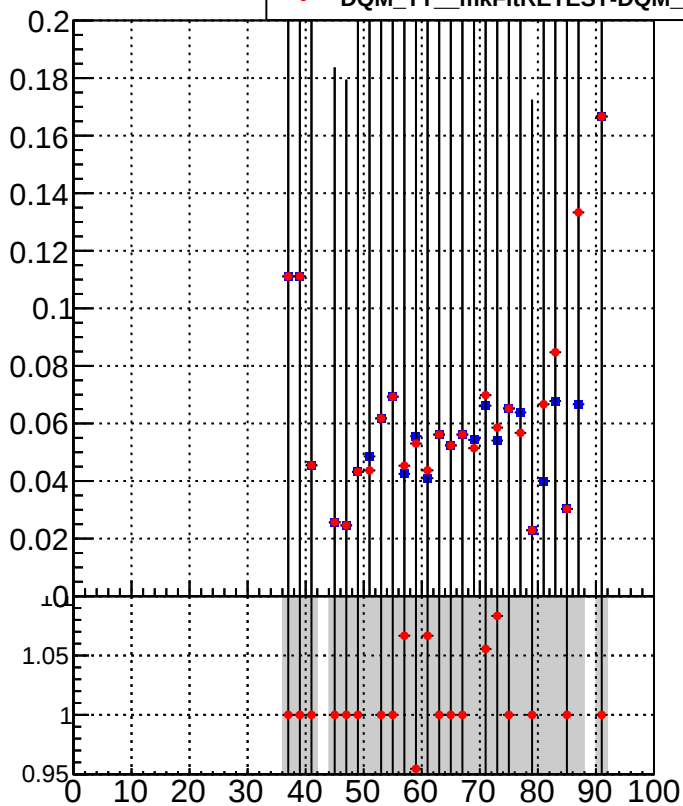
—■— DQM_TT_mkFit-DQM_ —●— DQM_TT_mkFitRETEST-DQM_
