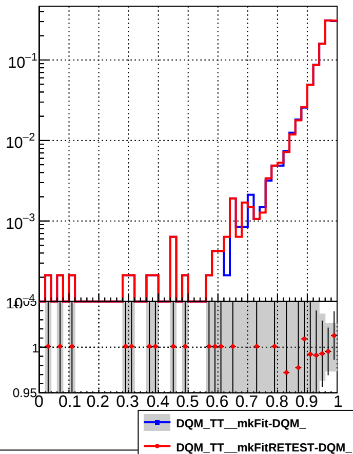
RecoPVAssoc2GenPVMatched_missing
