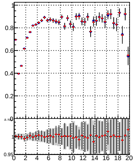
Fake rate vs. \text{DQM\_TT\_mkFit-DQM} \text{DQM\_TT\_mkFitRETEST-DQM}
