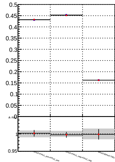
Fake rate vs. —●— DQM_TT_mkFit-DQM —●— DQM_TT_mkFitRETEST-DQM
