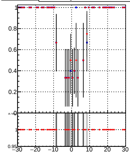
Fake rate vs \eta
