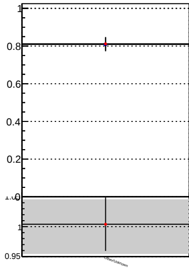
Fake rate vs. DQM_TT_mkFit-DQM DQM_TT_mkFitRETEST-DQM
