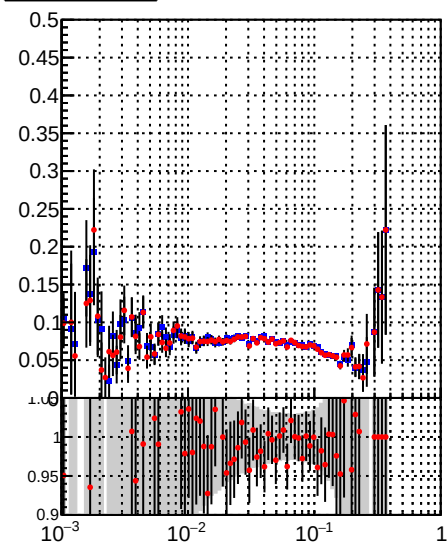
Legend: DQM_TT_mkFit-DQM (blue squares) DQM_TT_mkFitRETEST-DQM (red circles) Fake rate vs
