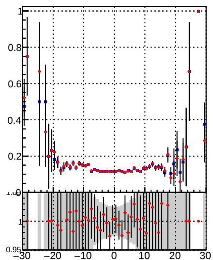
Fake rate vs \Delta d
