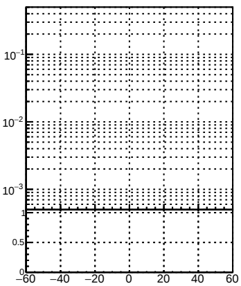
N of associated (recoToSim) looper tracks vs. sim PV
