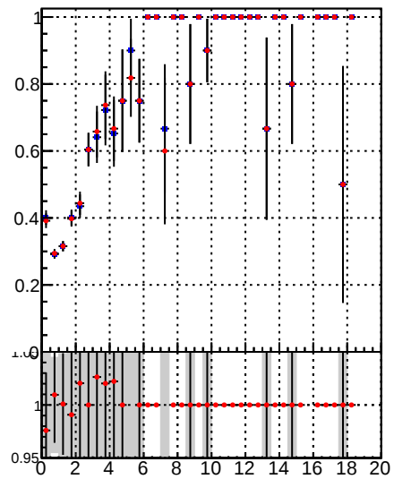
Fake rate vs. DQM_TT_mkFit-DQM DQM_TT_mkFitRETEST-DQM
