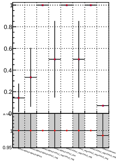
Fake rate vs. \text{DQM\_TT\_mkFit-DQM} \text{DQM\_TT\_mkFitRETEST-DQM}
