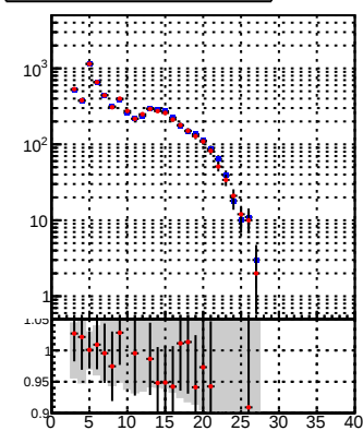
—•— DQM_TT_mkFit-DQM_ —•— DQM_TT_mkFitRETEST-DQM_ N of reco track vs hit
