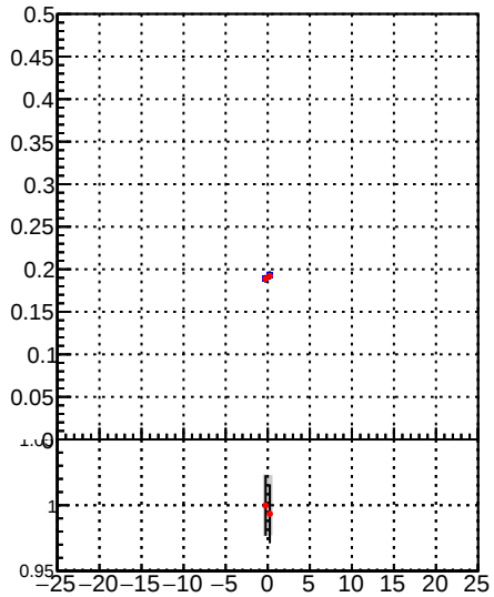
Fake rate vs d —●— DQM_TT_mkFit-DQM —●— DQM_TT_mkFitRETEST-DQM
