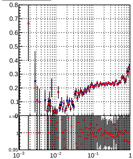
Legend: DQM_TT_mkFit-DQM_ (blue squares), DQM_TT_mkFitRETEST-DQM_ (red circles)
