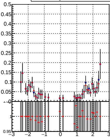
—■— DQM_TT_mkFit-DQM_ —●— DQM_TT_mkFitRETEST-DQM_
