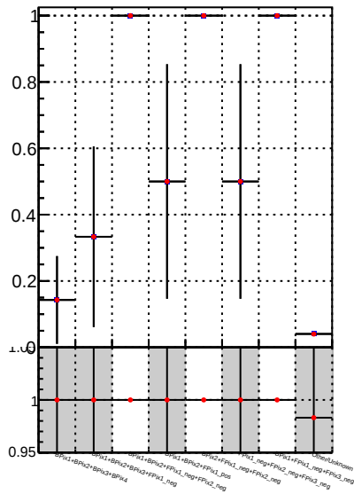
Fake rate vs. \bullet DQM_TT_mkFit-DQM \bullet DQM_TT_mkFitRETEST-DQM
