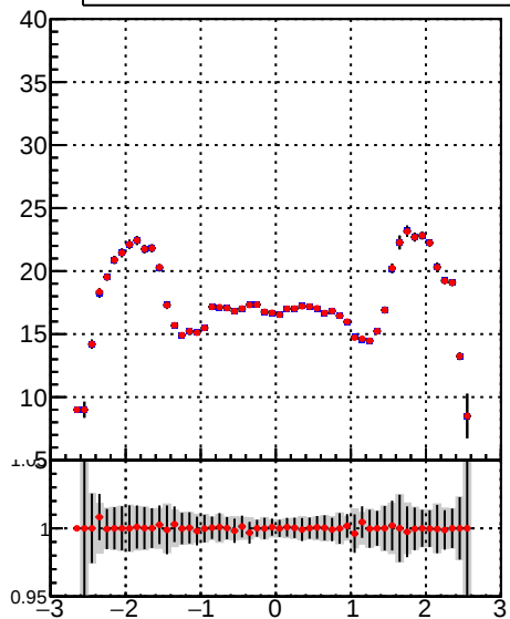
mean hit — DQM_TT_mkFit-DQM_ — DQM_TT_mkFitRETEST-DQM_
