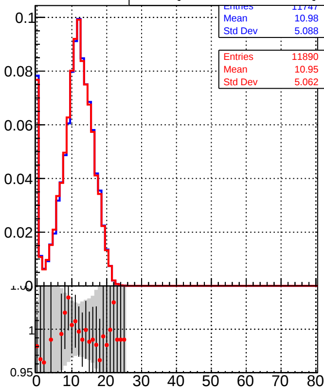
Legend: DQM_TT_mkFit-DQM_ DQM_TT_mkFitRETEST-DQM_
