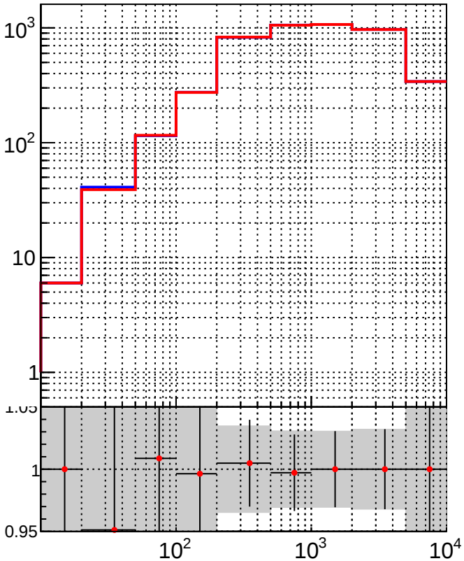
RecoAssoc2GenPVMatched_Pt2
