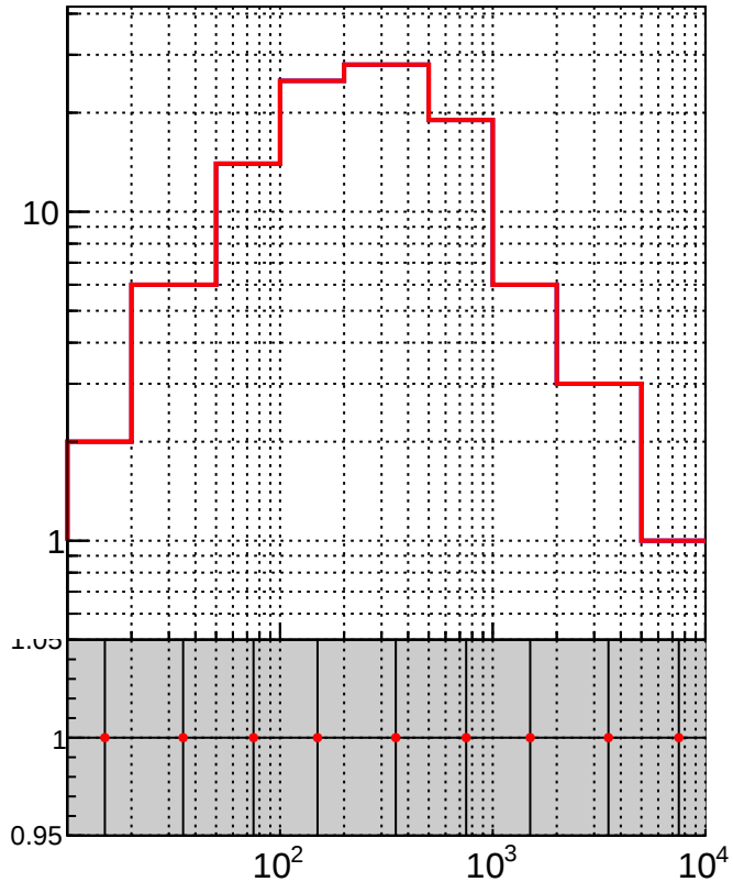
RecoAssoc2GenPVMatchedNotHighest_Pt2
