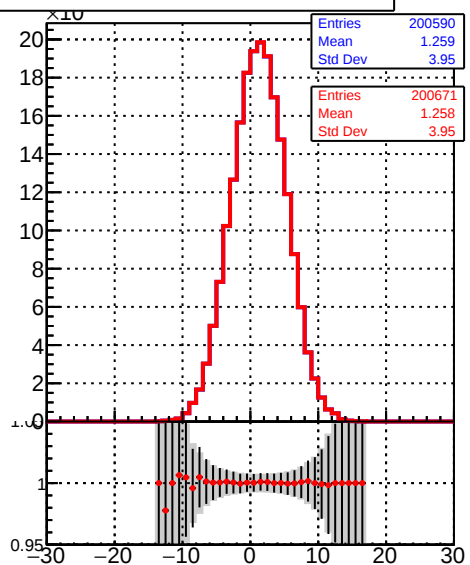
ReconstructedAllAssoc2Gen_NumTracks
