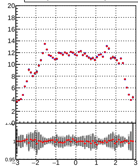
mean hit
