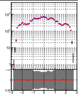
N of reco track vs \eta DQM_TT_mkFit-DQM N of reco track vs \eta DQM_TT_mkFitRETEST-DQM
