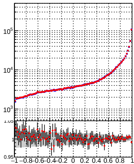
N of associated tracks (recoToSim) vs MVA1
