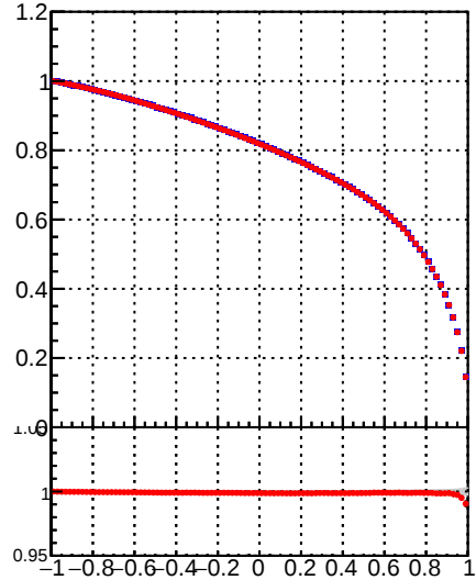
Efficiency (tracking eff factorized out) vs. MVA1
