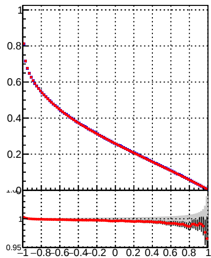
Fake rate vs. MVA1
