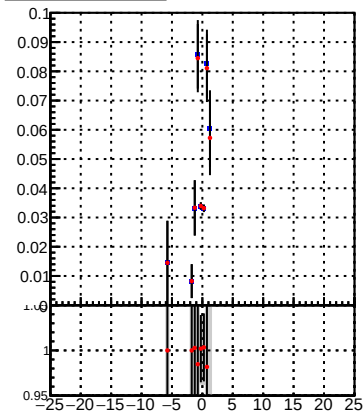
Efficiency vs Dxy(PV) plot comparing DQM_TT_mkFit-DQM_ (black line) and DQM_TT_mkFitRETEST-DQM_ (red line).
