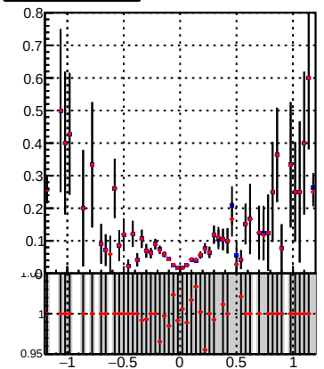
Efficiency vs Dz(PV) plot comparing DQM_TT_mkFit-DQM_ (black line) and DQM_TT_mkFitRETEST-DQM_ (red line).
