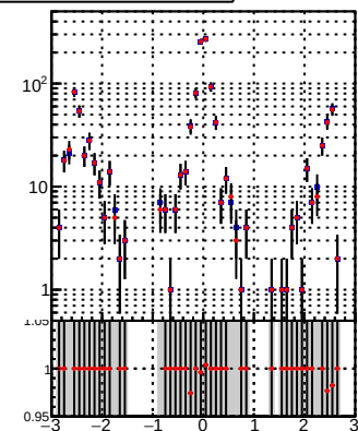
N of associated (recoToSim) tracks vs \eta DQM TT mkFit-DQM DQM TT mkFitRETEST-DQM
