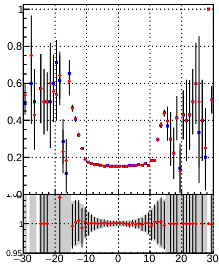
—•— DQM_TT_mkFit-DQM_ —•— DQM_TT_mkFitRETEST-DQM_
