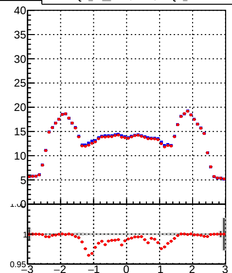
mean hit Legend: DQM_TT_mkFit-DQM_ (blue line), DQM_TT_mkFitRETEST-DQM_ (red line)
