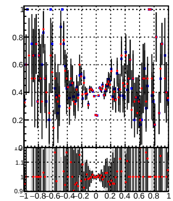
—●— DQM_TT_mkFit-DQM_ —●— DQM_TT_mkFitRETEST-DQM_
