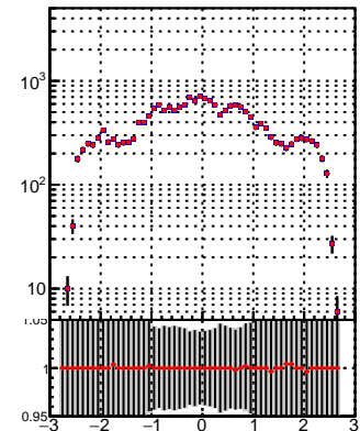
—•— DQM_TT_mkFit-DQM —•— DQM_TT_mkFitRETEST-DQM_
