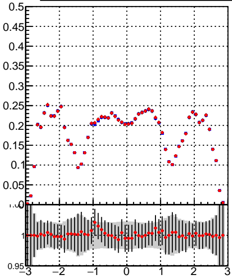
/data2/legianni/BDT-vs-DNN/real-BDT/CMSSW_13_0_0_pre4/src/runrem/DQM_TT_mkFit_ DQM_TT_mkFitRETEST3_
