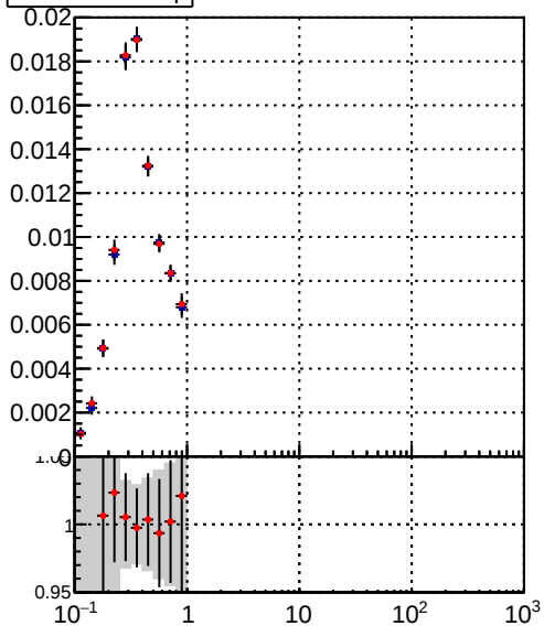
/data2/legianni/BDT-vs-DNN/real-BDT/CMSSW_13_0_0_pre4/src/runrem/DQM_TT_mkFit_ DQM_TT_mkFitRETEST3_
