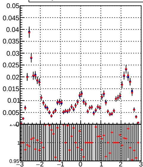
/data2/legianni/BDT-vs-DNN/real-BDT/CMSSW_13_0_0_pre4/src/runrem/DQM_TT_mkFit_ DQM_TT_mkFitRETEST3_
