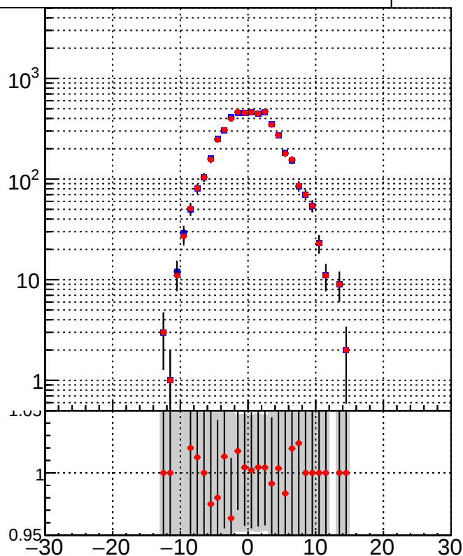
/data2/legianni/BDT-vs-DNN/real-BDT/CMSSW_13_0_0_pre4/src/runrem/DQM_TT_mkFit_ DQM_TT_mkFitRETEST3_
